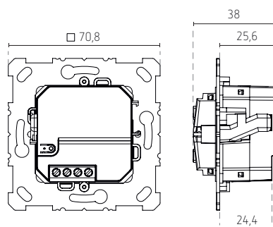
9080026, bascule simple
