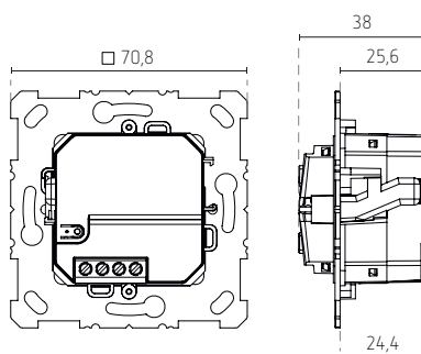
9080026, bascule simple
