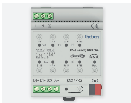
DALI Gateway S128 KNX
