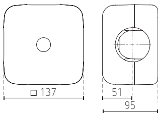
LK187109, Isolerende behuizing DN 25-32
