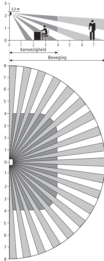
PresenceLight 180
