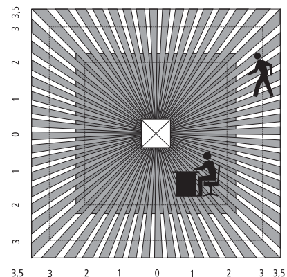
PresenceLight 360
