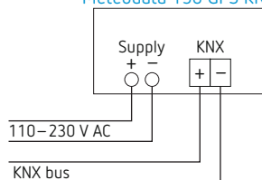
Meteodata 150 GPS KNX
