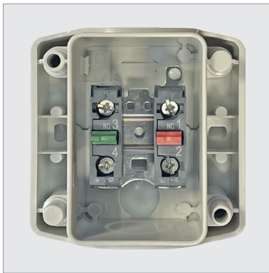
EMERGENCY STOP
