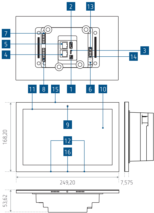
Dimensions (mm)
