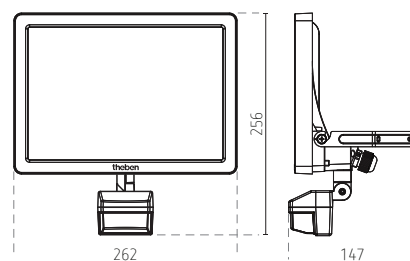
+ theLeda B dual sensor
