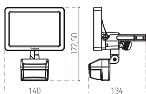
+ theLeda B dual sensor
