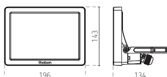
theLeda B30 dual | theLeda B50 dual
