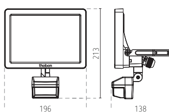
+ theLeda B dual sensor
