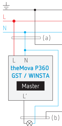
GST-connector
